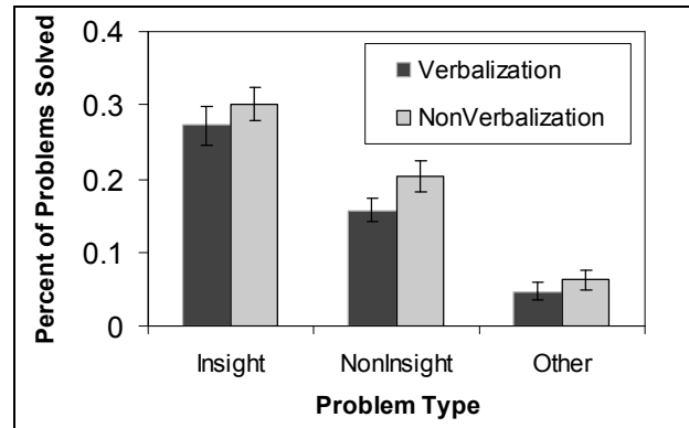
Figure 1: Solution rates of attempted problems. Mean percentage of attempted problems solved with insight, noninsight, or other while verbalizing and while not verbalizing. Error bars indicate one standard error.
